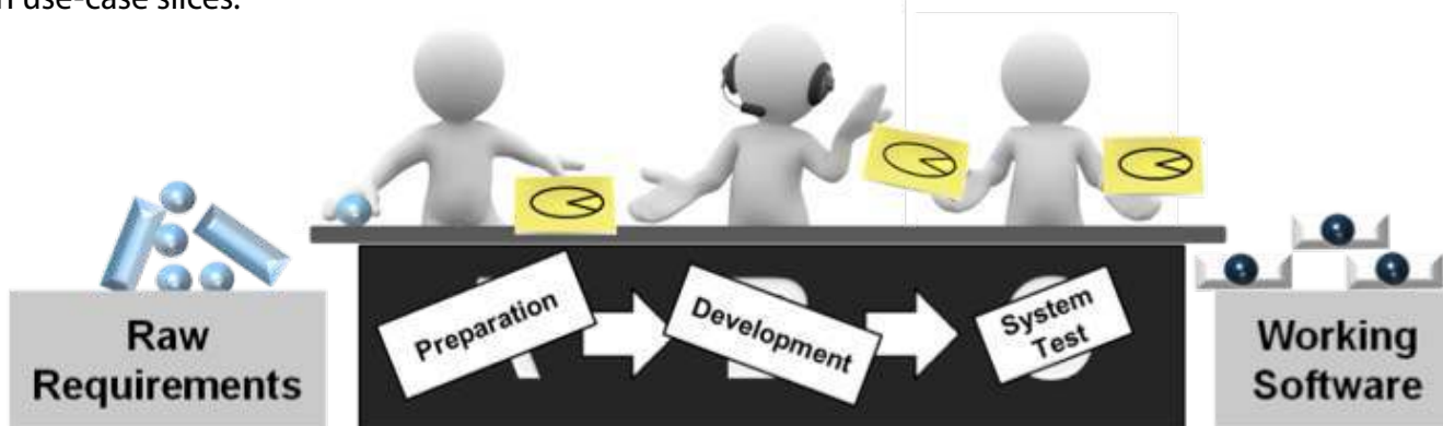
FIGURE 19: ONE-PIECE FLOW FOR SOFTWARE DEVELOPMENT WITH USE-CASE SLICES
